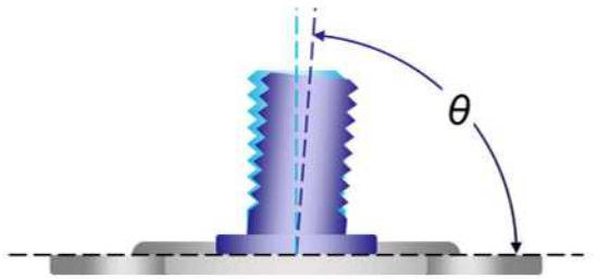
Perpendicularity
